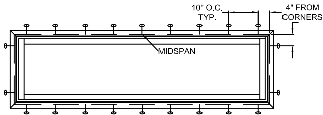
TYPICAL ELEVATION WITH FASTENER SPACING
